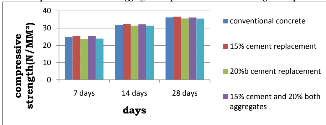
Comparison For Different Aggregates Replacement With Percentages Compressive Strength
